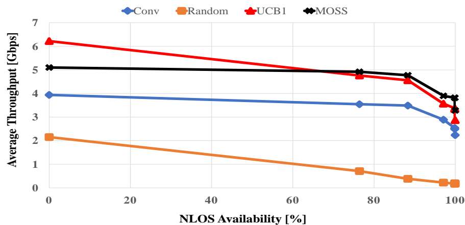
Figure 6. Average Throughput vs NLOS availability for 60 Devices
