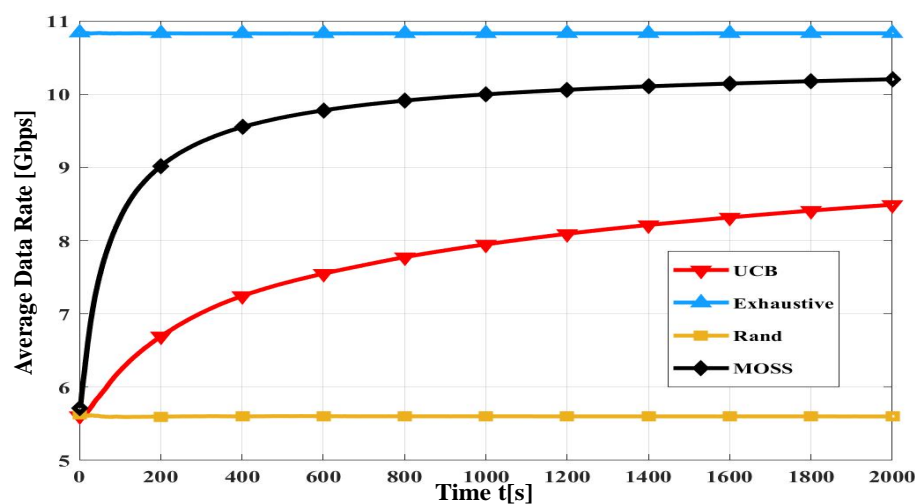
Figure 7. UCB and MOSS convergence vs Horizon
