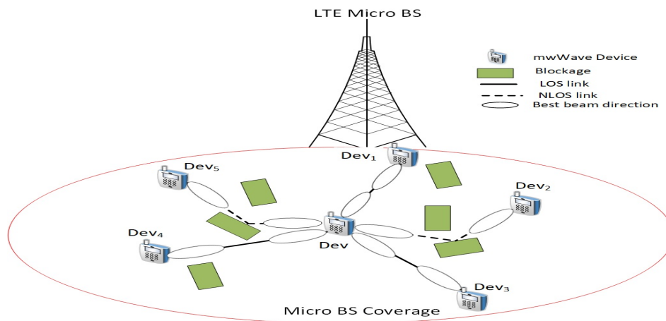
Figure 4. Utilized mmWave D2D System Model
