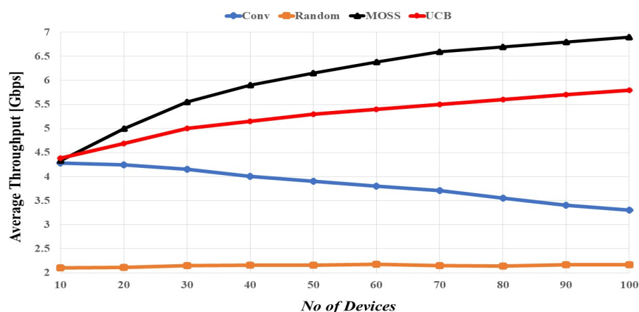
Figure 5. Average Throughput comparisons at no blockage
