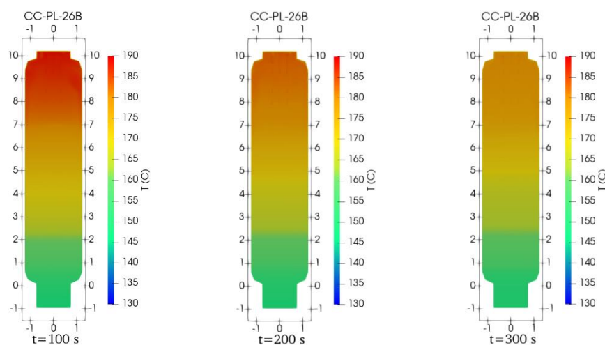
(b) Cross-section temperature contour: CFD simulation-CHT_SSTKO
