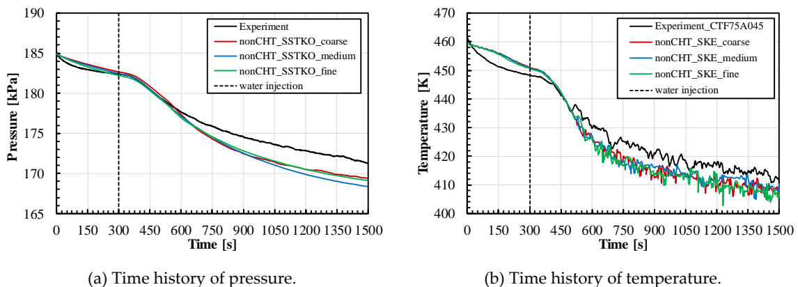
Figure 6. Comparison of the measured pressure and temperature (black lines) with the numerical CFD on the coarse mesh (red lines), medium mesh (blue lines), and fine mesh (green lines).
