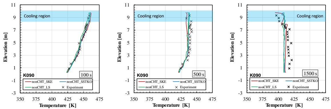
Figure 8. Comparison of the measured and numerically predicted temperature profile at K090.
