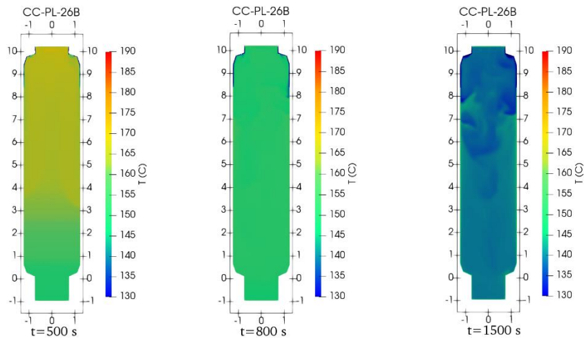
(b) Cross-section temperature contour: CFD simulation-CHT_SSTKO
