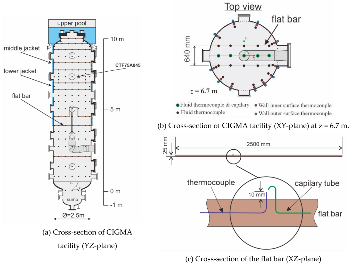
Figure 1. The schematic drawing of CIGMA facility at JAEA.
