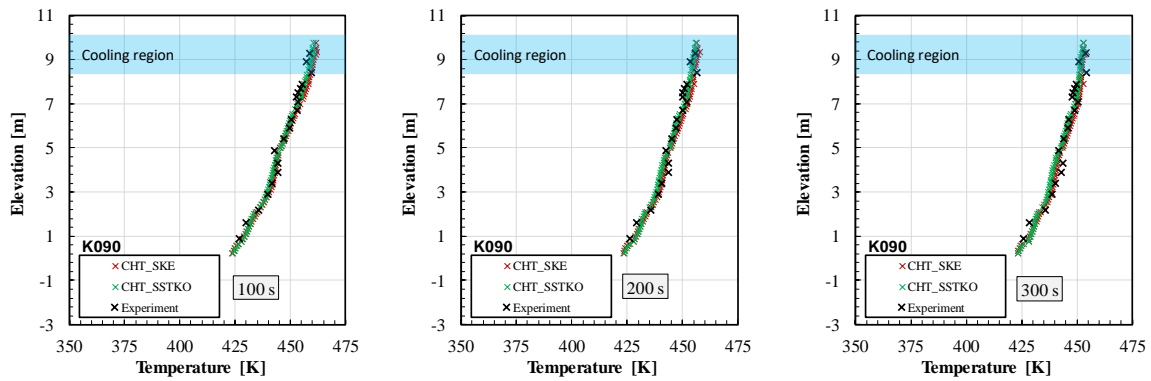
(a) Temperature profile at K090 before water injection in the upper pool and middle jacket.
