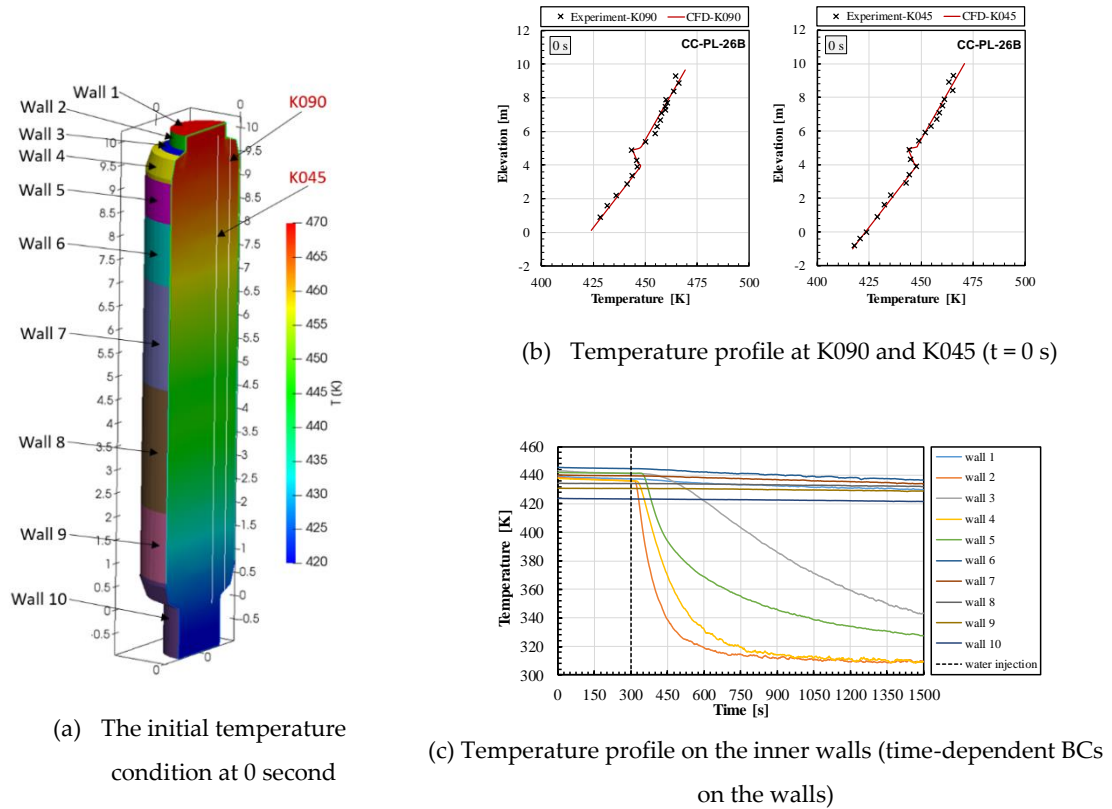
Figure 3. Temperature initial condition inside the vessel and the boundary conditions at the walls.
