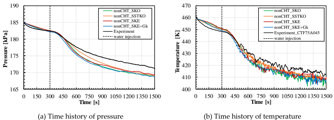
Figure 9. Time history of pressure and temperature as measured (black line) and numerically predicted by means of different turbulence models (colored lines).
