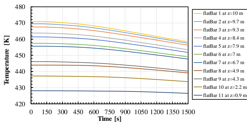
Figure 13. The predicted of the average temperature on the flat bars by means of SST k-\omega turbulence model with CHT.
