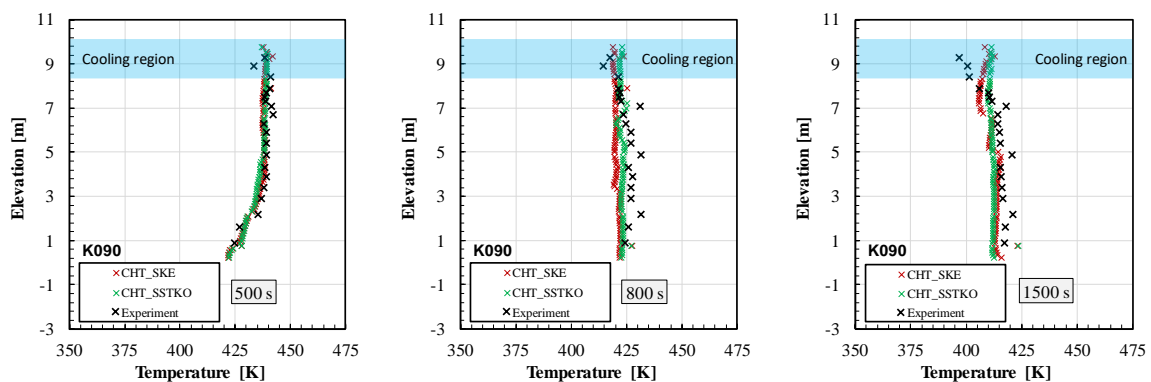
(b) Temperature profile at K090 after water injection in the upper pool and middle jacket.
