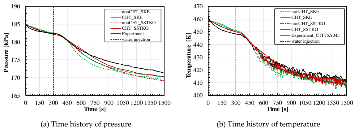
Figure 10. Time history of pressure and temperature as measured (black line) and numerically predicted by means of different turbulence models with CHT (solid lines) and without CHT (dash lines).
