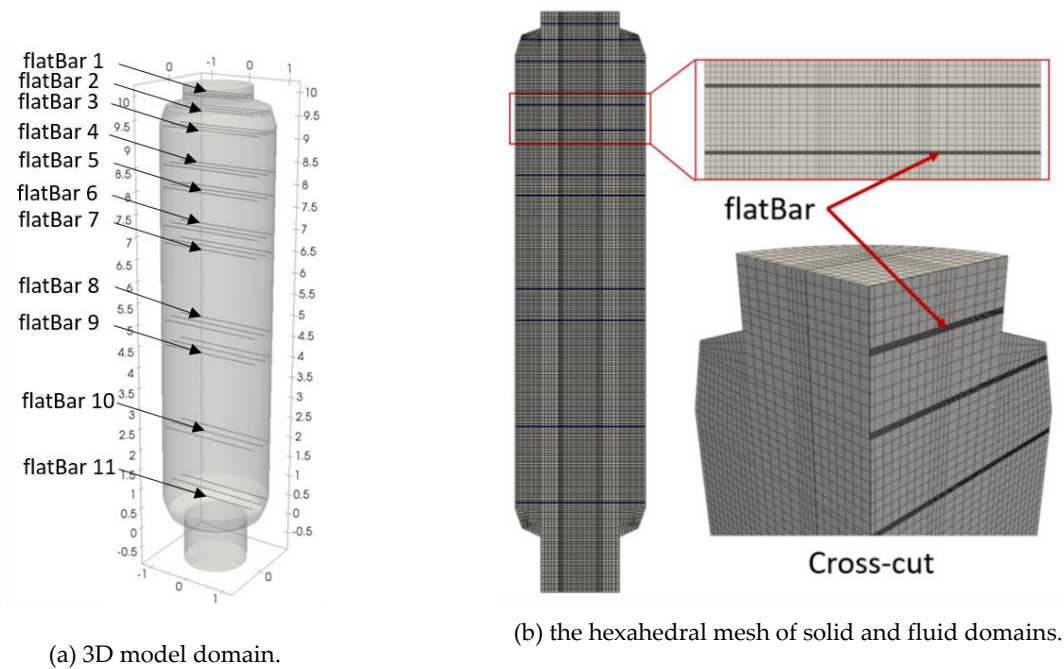
Figure 2. 3D model geometry and mesh.
