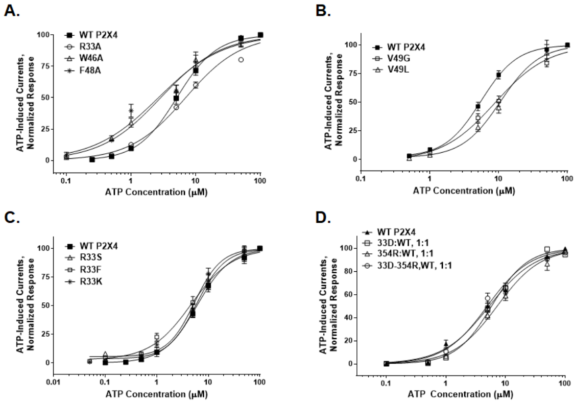
Supplementary Figure A1. ATP concentration-response curves for WT and select P2X4R mutants. (a) There was a right-shift in the ATP concentration-response curves for R33A and F48A but not for W46A mutant compared to that of the WT receptor. (b) A right-shift in the ATP concentration-response curves shown for V49G and V49L mutants. (c) Position 33 mutants demonstrated WT-like ATP concentration responses. (d) WT-like ATP concentration responses for position 33 and 354 reciprocal mutant:WT receptor mixtures.
