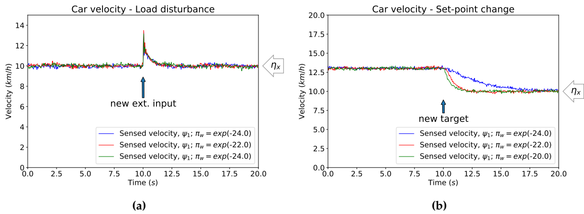
Figure 3. Different responses to load disturbances and set-point changes. The simulations were 300s long, with an external disturbance/different target velocity introduced at t = 150\text{s} . Here we report only a 20 seconds time window around the change in conditions. (a) The same load disturbance ( v = 3.0\text{km/h}^2 ) is applied with varying expected process precisions \pi_{\tilde{w}} where \pi_w = \{\exp(-24), \exp(-22), \exp(-20)\} . Expected sensory log-precisions \pi_{\tilde{z}} are fixed over the duration of the simulations, with \mu_{\gamma_z} = 1 . (b) A similar example for changes in the target velocity of the car, from \eta_x = 13\text{km/h} to \eta_x = 10\text{km/h} , tested on varying expected process precisions \pi_{\tilde{w}} where \pi_w = \{\exp(-24), \exp(-22), \exp(-20)\} .
