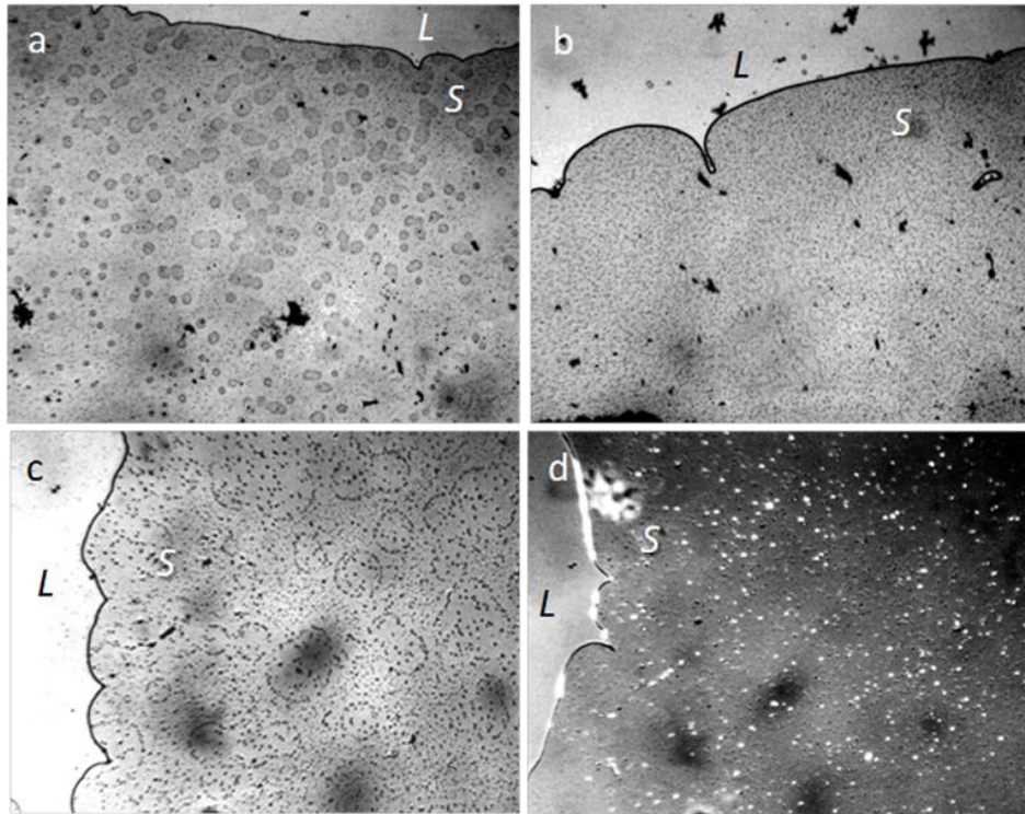
Figure 17. Structure of deposits in the drying film of aqueous solutions of NaCl: a - 3%; b - saturated; c and d - 4%. The width of frames a and b is 3 mm; c and d - 1 mm; d - a picture in a semi-dark field; L is the evaporating liquid phase.
