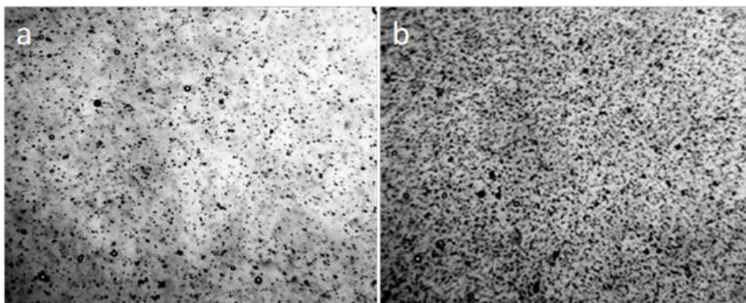
Figure 14. Microscopy of the open surface of an aqueous solution of coffee, poured into a Petri dish, at different temperatures: +20^\circ\text{C} (a) and +4^\circ\text{C} (b). Increase in density and decrease in the size of coacervate structures upon solution cooling. The width of each frame is 3 mm.
