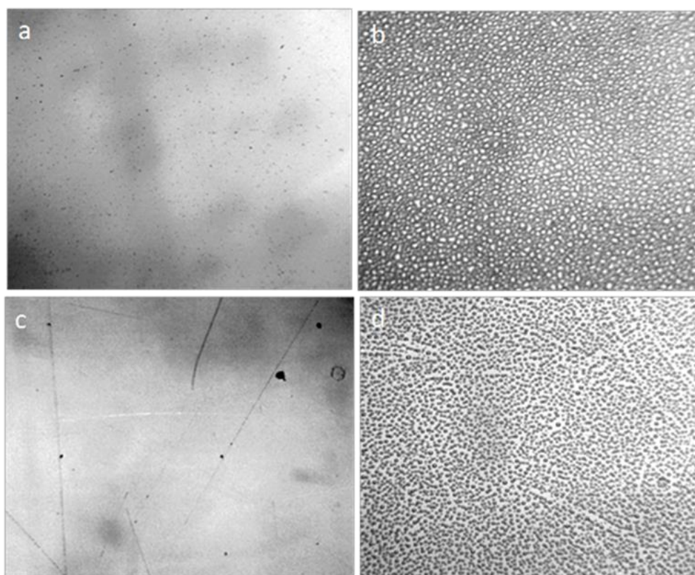
Figure 9. The formation of regular icy patterns on the surface of the dry glass (a) and dry plastic (c), after incubating them in the freezer at -20^{\circ}\text{C} (b and d, respectively). The width of each frame is 3 mm.
