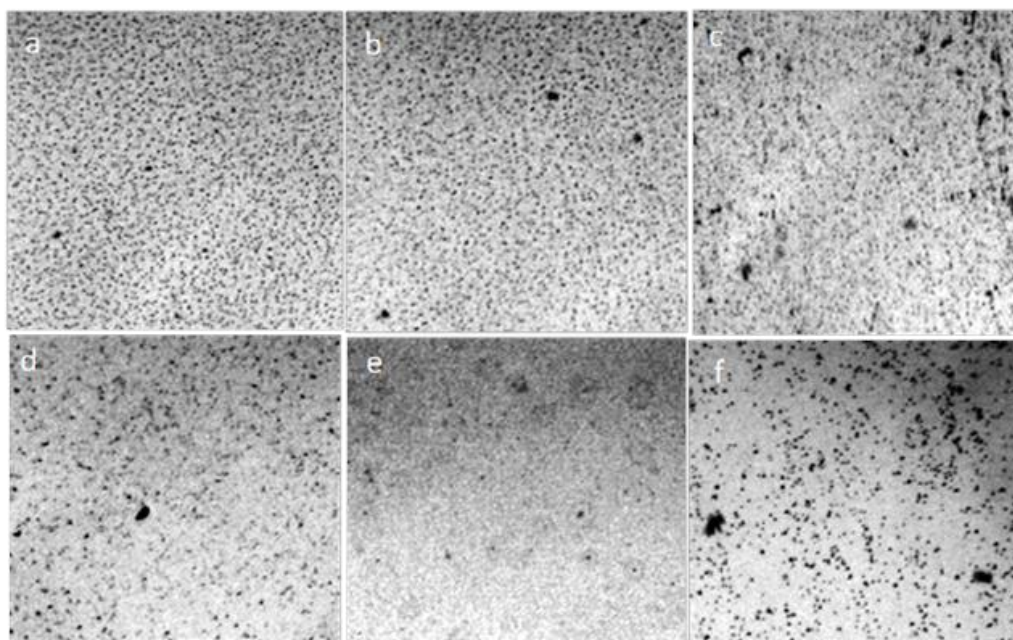
Figure 15. Structure of liquids in thin films ( \sim 8 \mu\text{m} ), enclosed between the objective and cover slip: a - distilled water; b - 1% NaCl solution; c - 2% NaCl solution; d - 3% NaCl solution; e - 4% NaCl solution; f is a saturated NaCl solution. Optical microscopy. The width of each frame is 1 mm.
