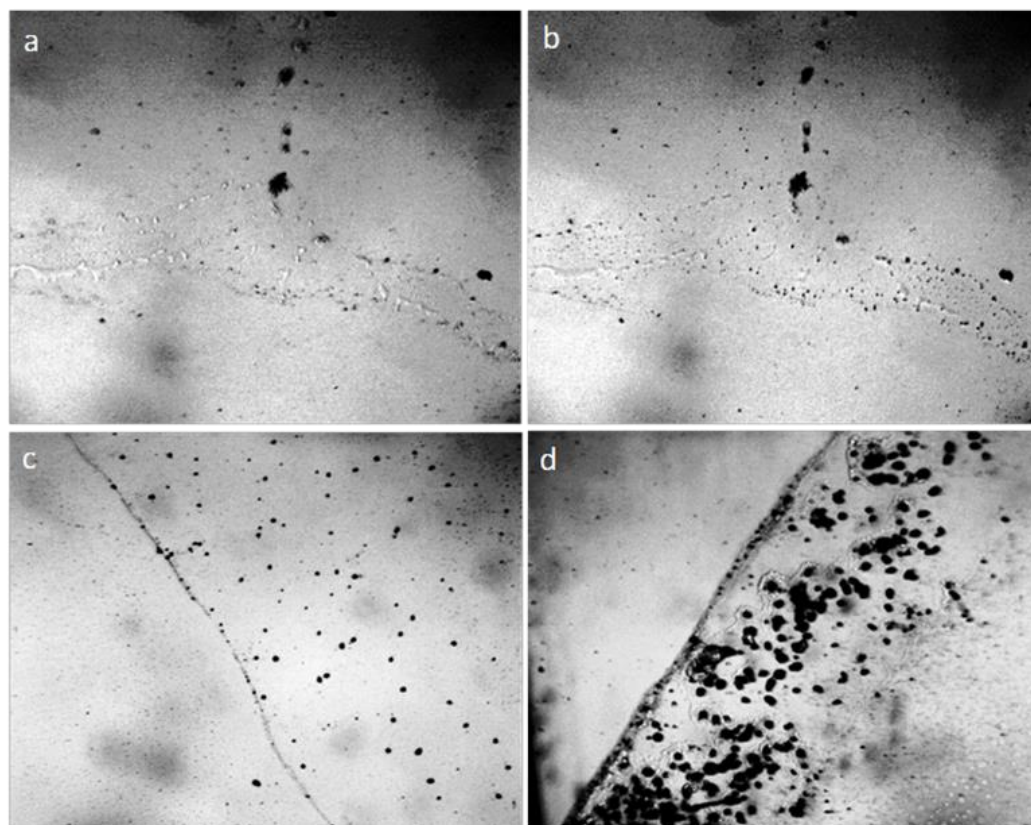
Figure 4. The edge of tap water film dried on the glass in the open air: a - after 5 days (focus on the upper boundary of liquid water droplets, b - focus on water-holding particles); c - crystal size after 7 days of drying; d - the size of the crystals after 14 days from the moment when the water was placed on the glass. The width of each frame is 3 mm.
