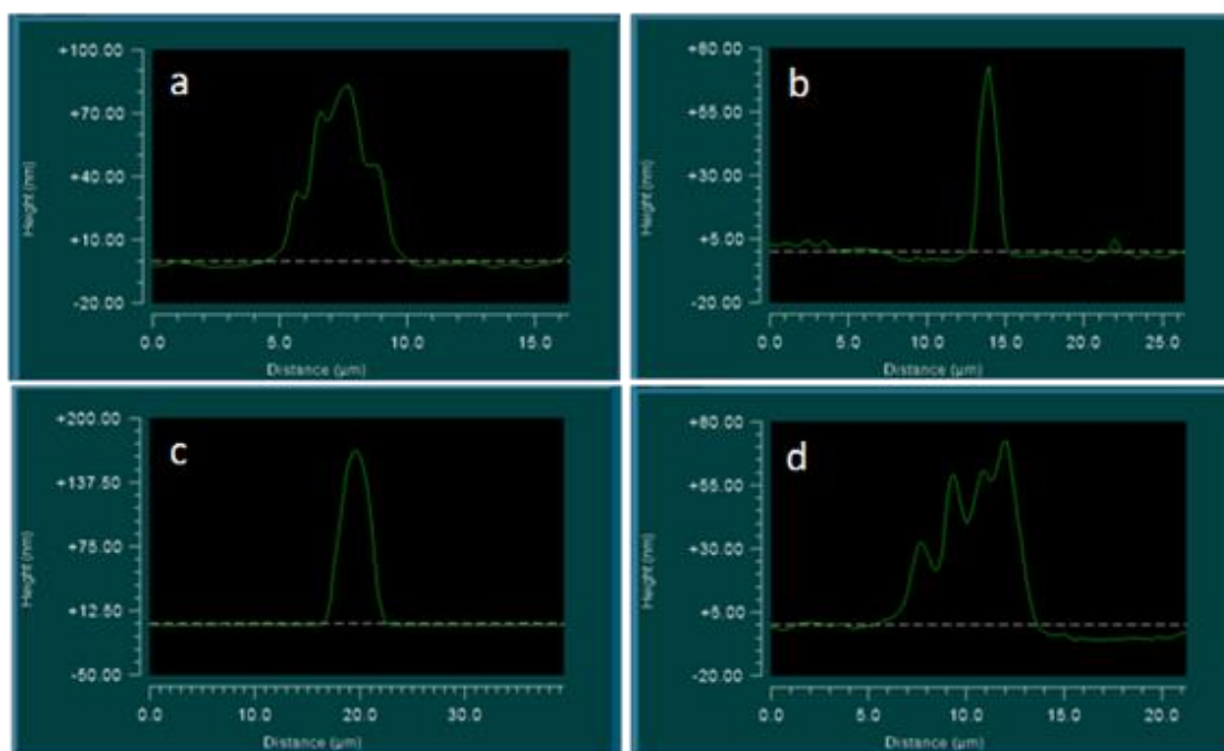
Figure 8. Samples of the crystal structure in the centre of the circles, covering the surface of a glass slide, according to interference microscopy.
