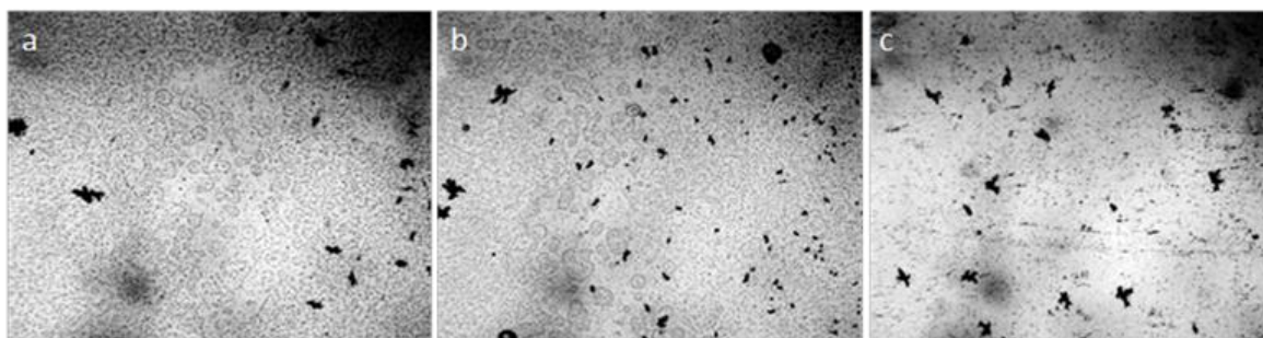
Figure 13. Coacervation of the dispersed phase of water in thin films ( \sim 8 \mu\text{m} ), enclosed between the objective and cover slip: a - distilled; b – tap water; c is b after boiling. Optical microscopy. The width of each frame is 3 mm.
