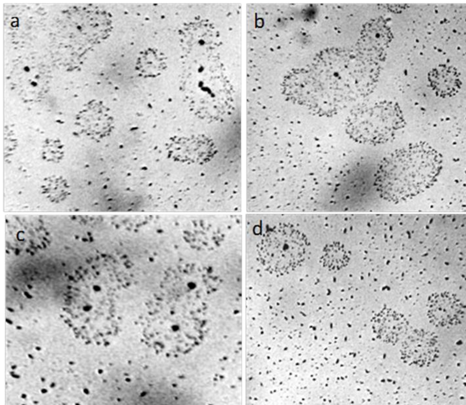
Figure 18. Coacervate structures of deposits in a dried film of 3% aqueous NaCl solution. The width of each frame is 0.25 mm.
