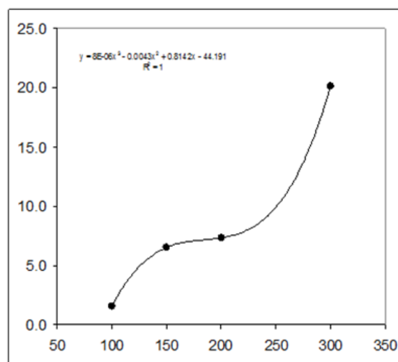
Figure 3. Results of chromatography-mass spectrometric analysis of a sample of a dried coffee solution for water content. X is the temperature of the sample (C degrees), and Y is the mass fraction of the liberated water (mass%) [36].
