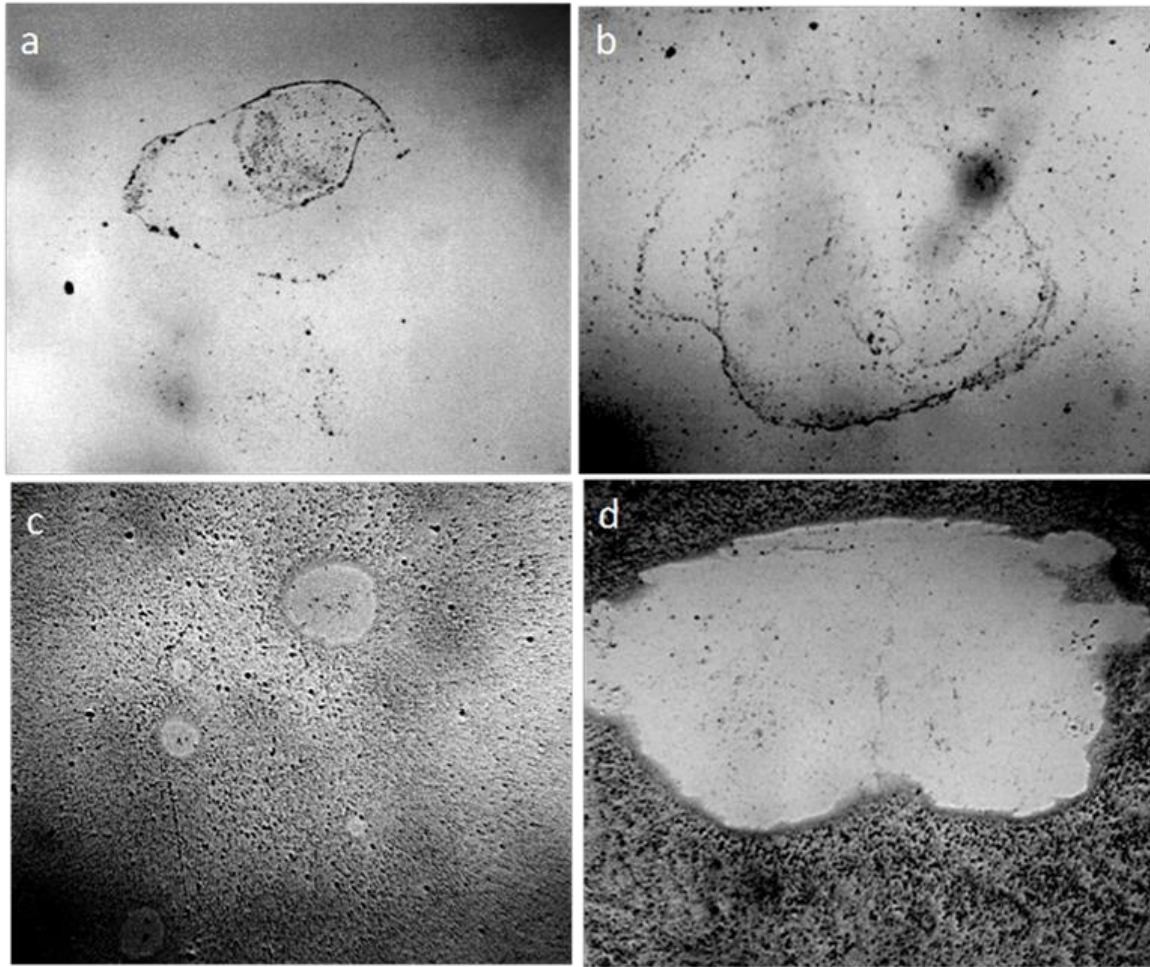
Figure 2. Fragments of dried out smears of the investigated liquids: a - distilled water; b - white dry wine; c and d are instant coffee. Agglomerates from the coalesced round structures are shown in Figure 1. The width of each frame is 3 mm.
