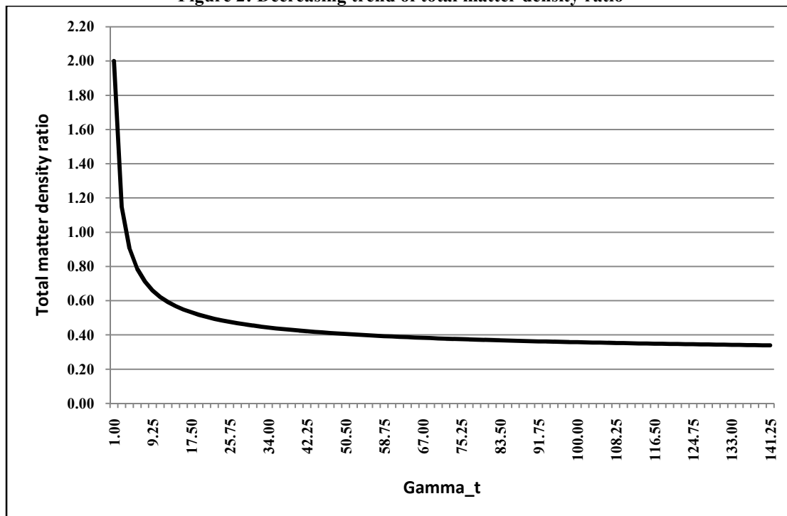
Figure 2: Decreasing trend of total matter density ratio
