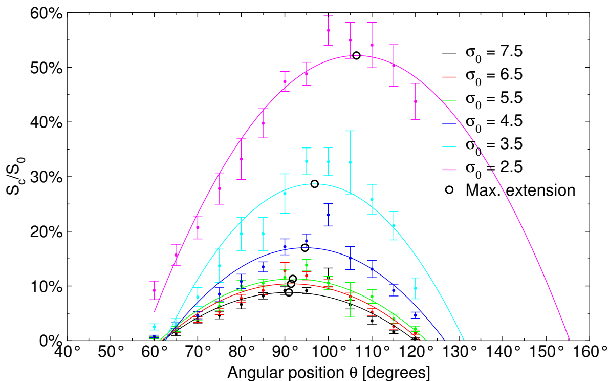
Figure 6. Cavity extension and corresponding root-mean-square fluctuations as a function of the propeller angle \theta and for \sigma_0 \in [2.5, 7.5] . The continuous lines are quadratic fit curves to the respective experimental data. The black circles indicate the location of the cavity maximum extension calculated from the fit function.
