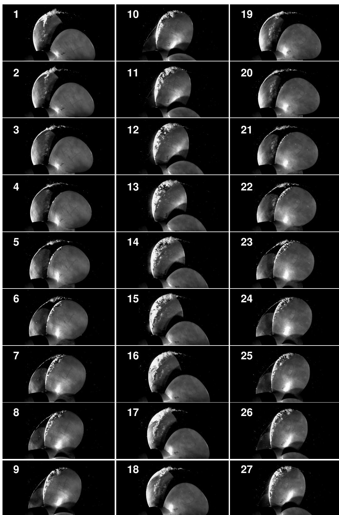
Figure 4. High-speed sequence of the cavitating propeller for \sigma_0 = 3.5 . Interframe time= 500 \mu\text{s} , angular step= 5.4^\circ . Flow is from left to right, and view is from propeller backface, portside. Wake generator is on the left.
