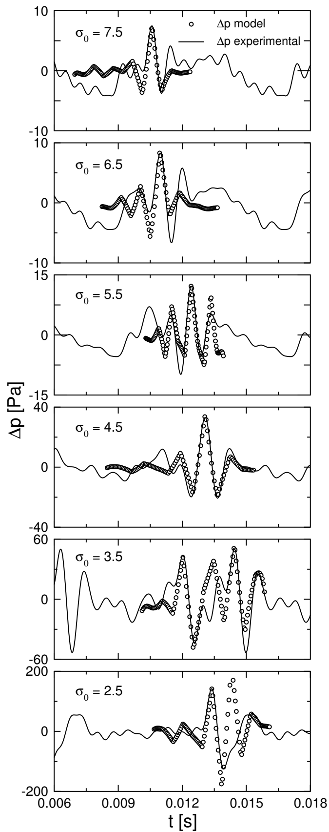
Figure 14. Comparison between measured \Delta p (—) and \Delta p estimated ( \circ ) from volume acceleration as per Eq. (11).
